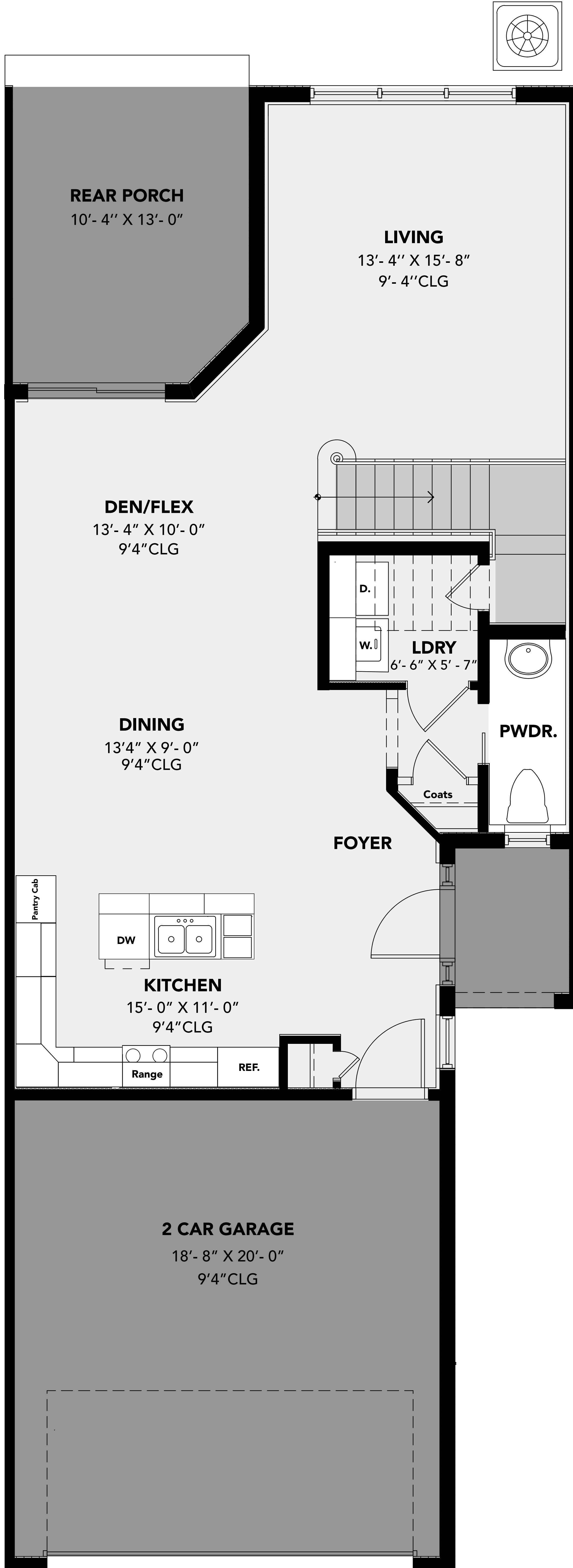
1ST FLOOR
